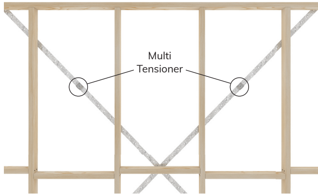
Figure 1: Multi Tensioner
